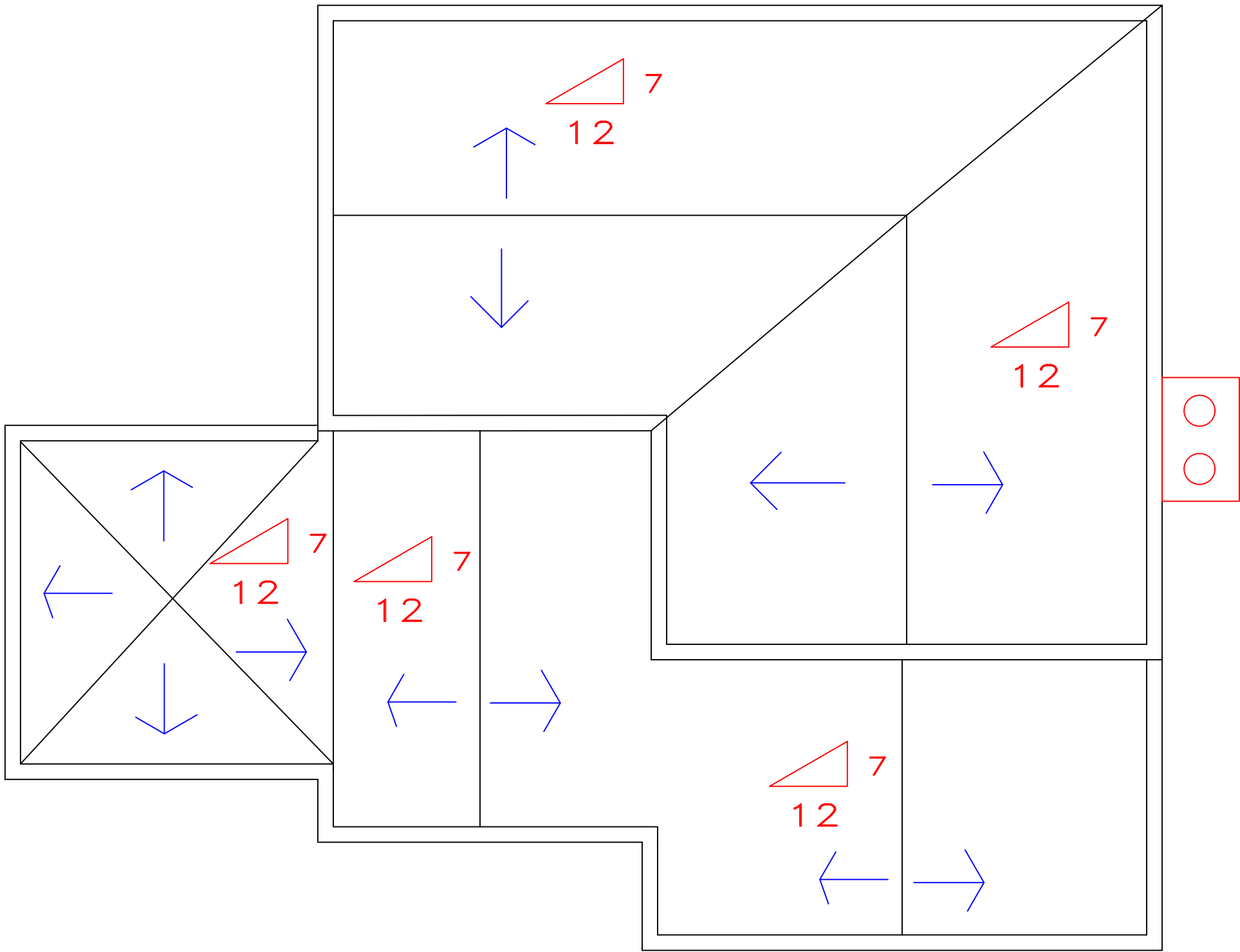
A 013 ROOF PLAN SCALE 1/4"=1'-0"
